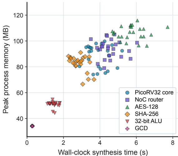
(b) Runtime and memory, same runs
