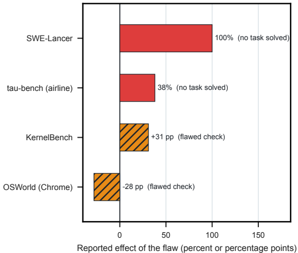
Agentic benchmark flaws (ABC audit)
