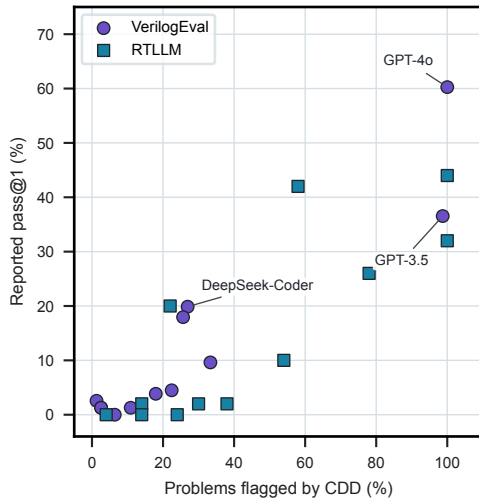
Verilog contamination flag vs. pass@1
