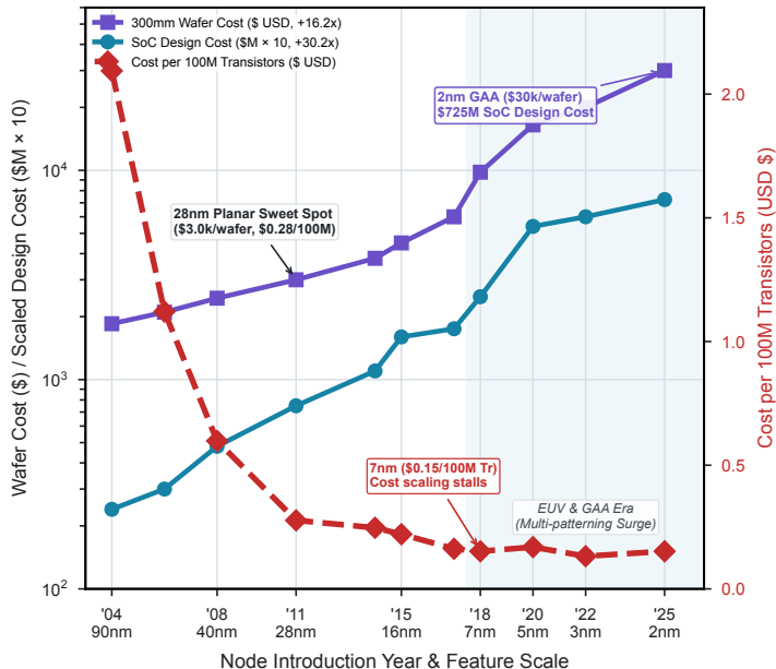
A. Foundry Wafer & Design Cost Inversion (90nm to 2nm)
