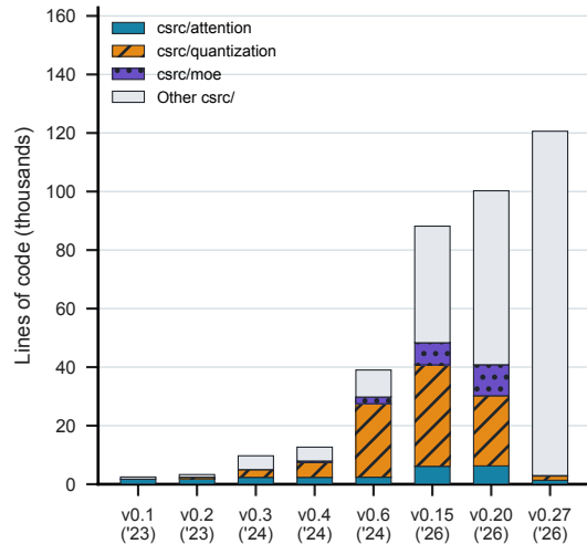
(c) vLLM native kernels (csrc/)
