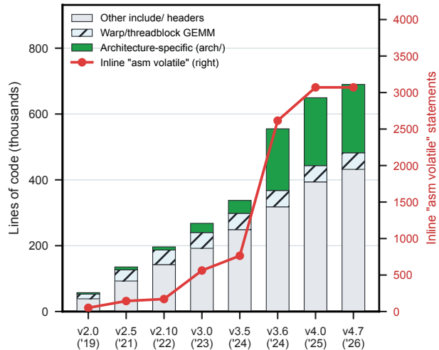
(a) CUTLASS headers
