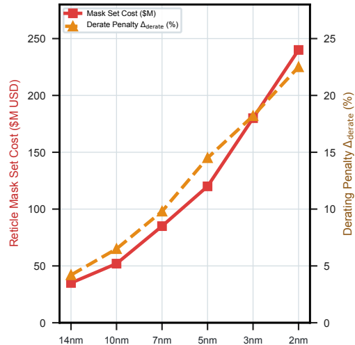
C. Mask Cost vs Derating
