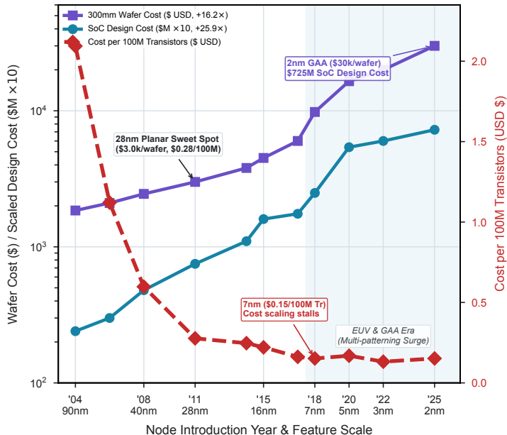
Panel A: Foundry Wafer & Design Cost Inversion (90nm to 2nm)
