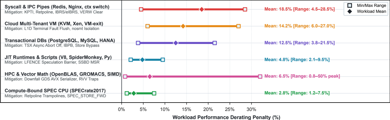
Panel B: Performance Tax Derating by Workload Class & Microarchitectural Mechanism
