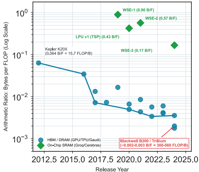
Panel B: Operational Intensity Wall (Byte/FLOP Collapse)
