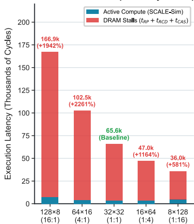
Panel A: Closed-Loop Latency Blowup
