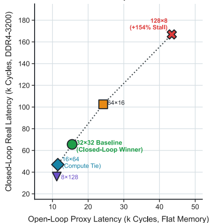
Panel C: Closed-Loop Pareto Inversion
