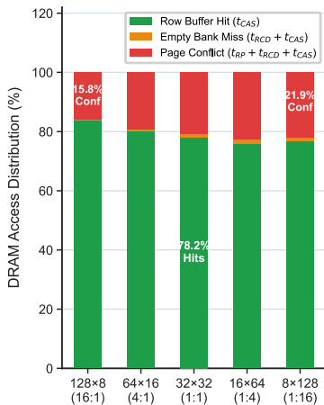
Panel B: Row-Buffer Conflict Breakdown
