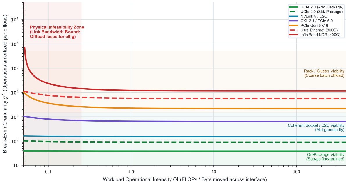
LogCA Break-Even Offload Frontiers Across Physical Interconnect Regimes
