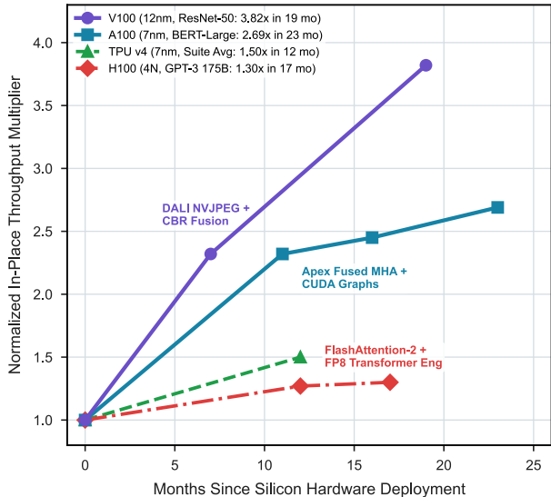
Panel A: The Fixed-Silicon Software Dividend
