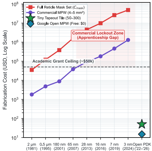
A. Physical Silicon Fabrication Cost Barrier
