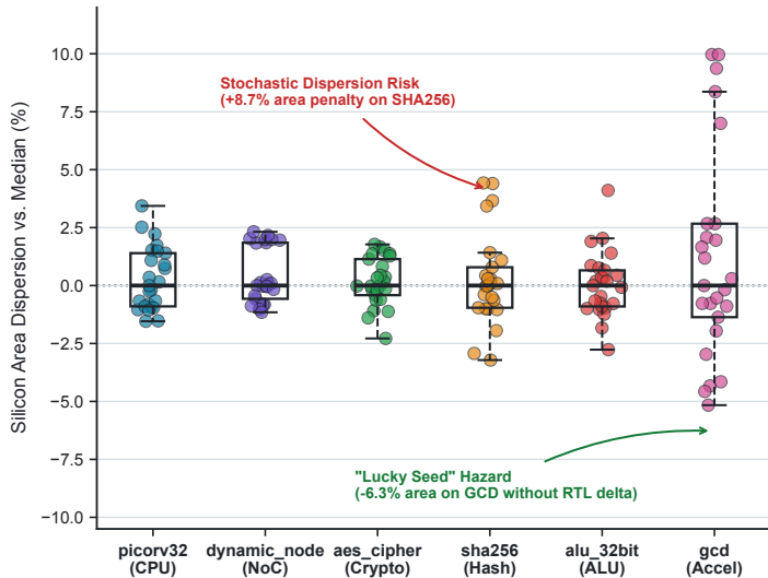
A: Area QoR Dispersion Across Logic Synthesis Pass Schedules
