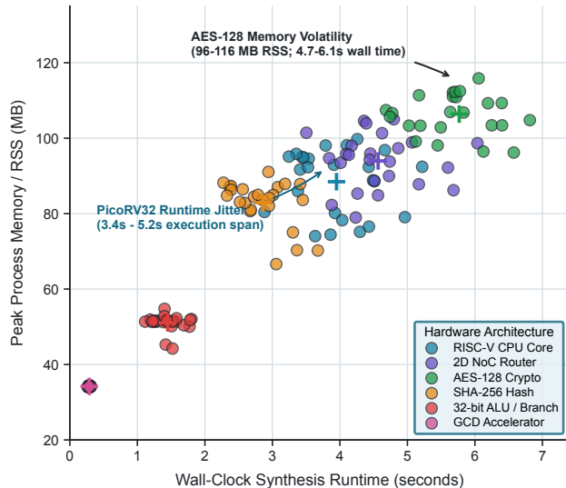
B: Tool Resource Footprint & Execution Jitter (150 Runs)
