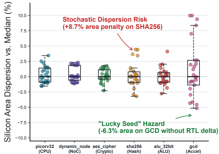
(a) Logic Synthesis Pass Dispersion
