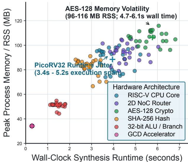
(b) Host Resource Footprint and Jitter
