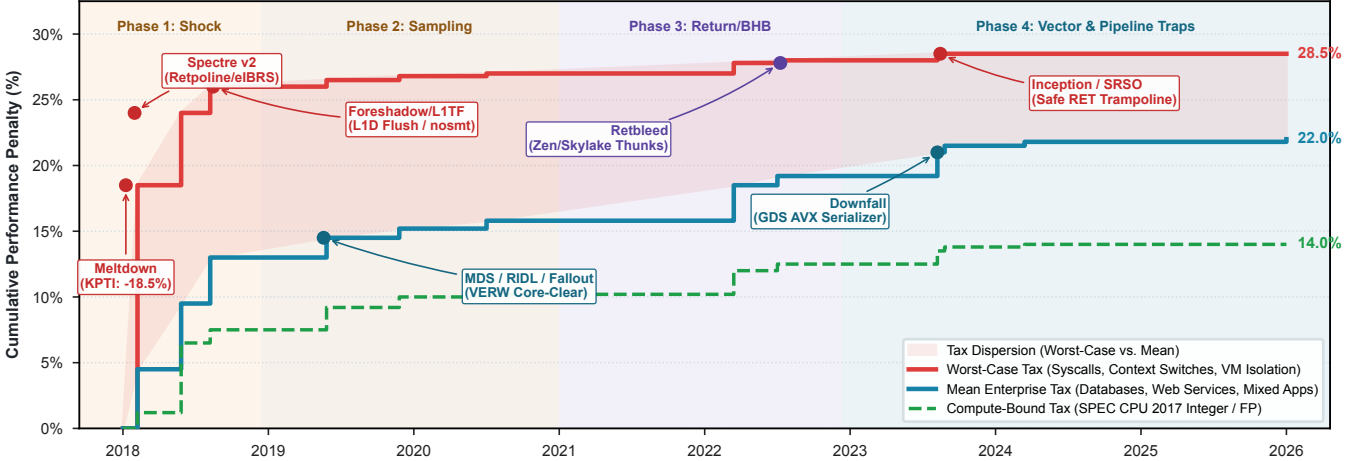
A. Longitudinal Vulnerability Timeline & Cumulative Speculative Execution Tax (2018–2026)
