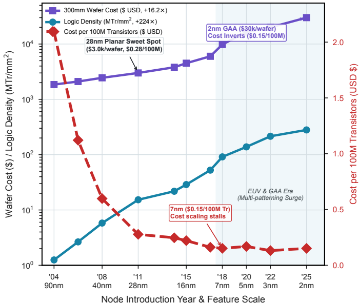
Panel A: Foundry Transistor Cost Inversion (28nm to 2nm)
