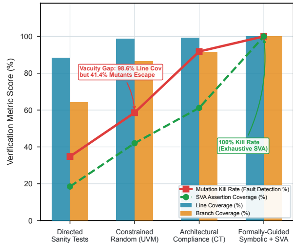
Panel B: The Testbench Vacuity Paradox (Coverage vs. Mutation Score)
