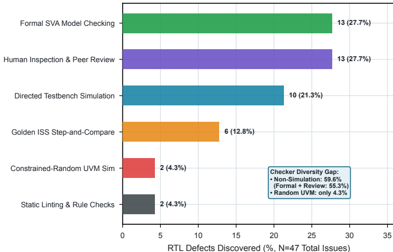
Panel A: Defect Discovery by Modality (OpenHW CV32E40P Audit)
