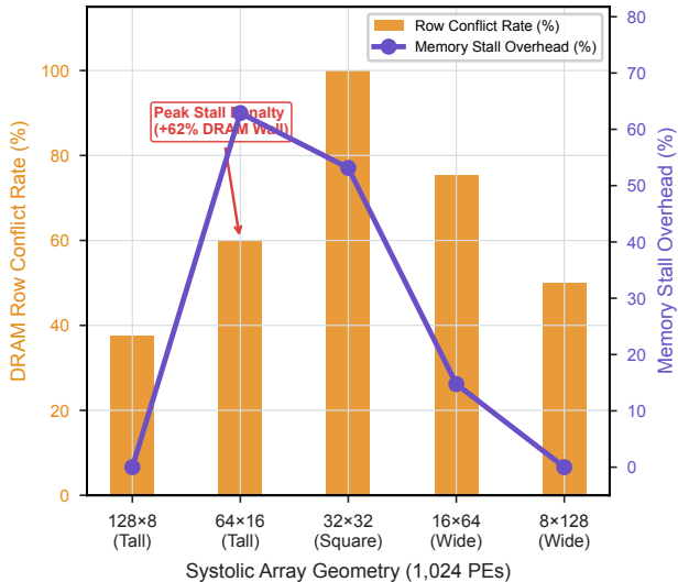
DRAM Bank Conflicts & Latency Inversion
