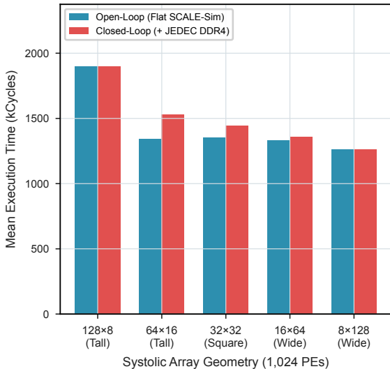
Open-Loop vs. Closed-Loop Execution Time
