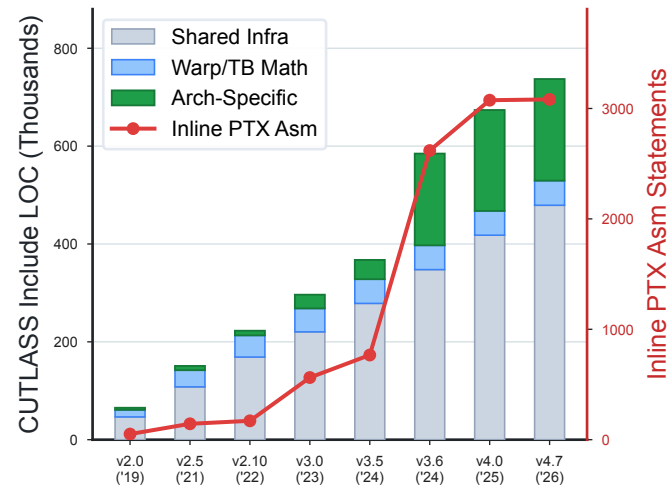
(a) CUTLASS Library source components
