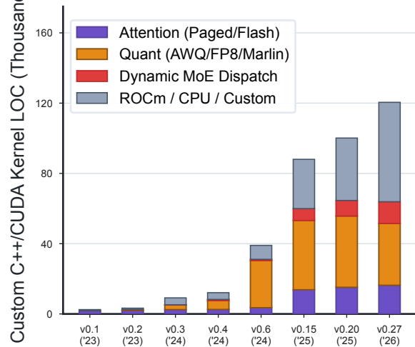
(c) vLLM Custom kernel source
