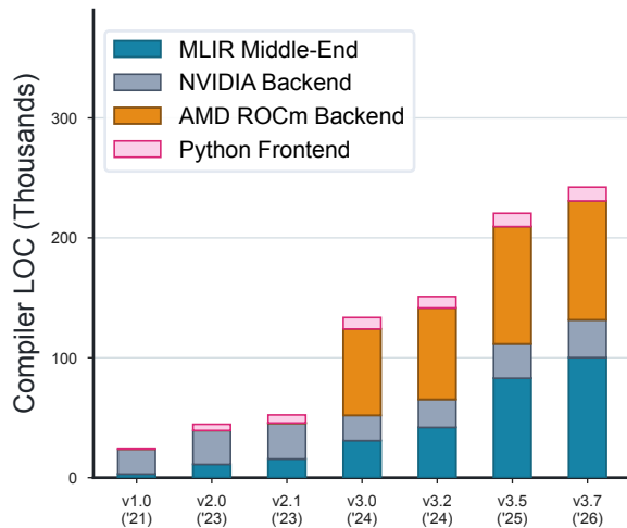
(b) Triton Compiler source components
