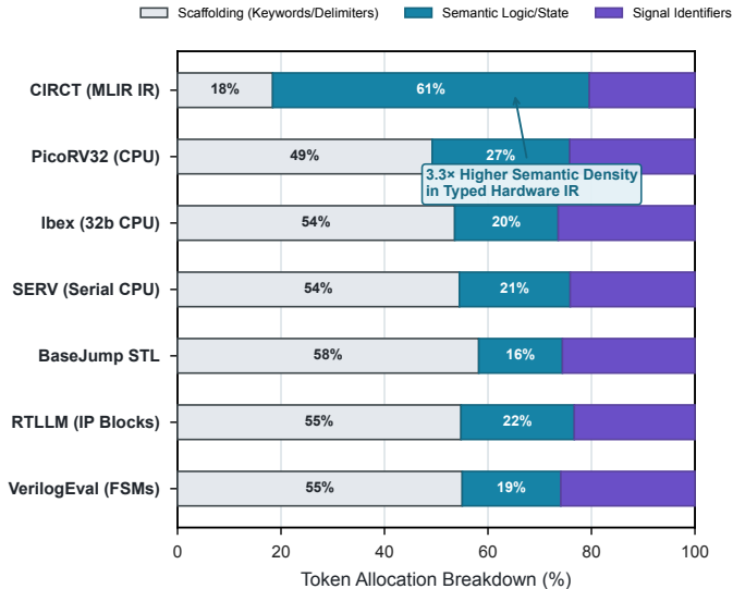
B. Syntactic Scaffolding vs. Semantic Density
