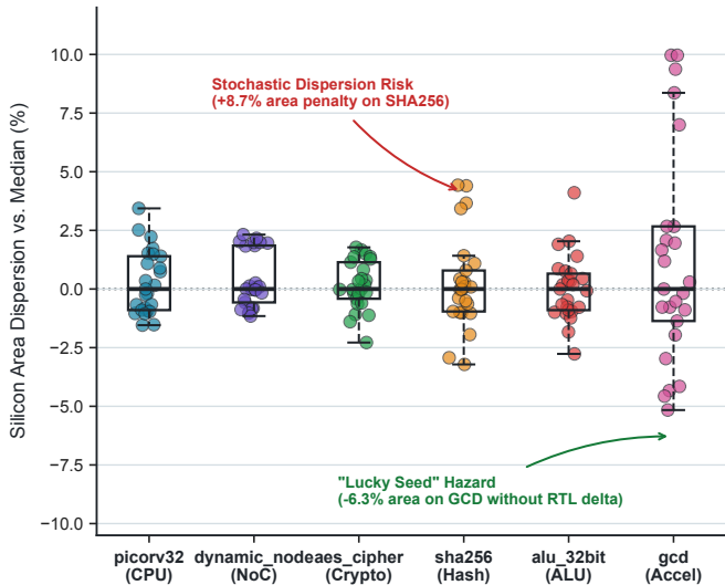
A: Area QoR Dispersion Across Logic Synthesis Pass Schedules
