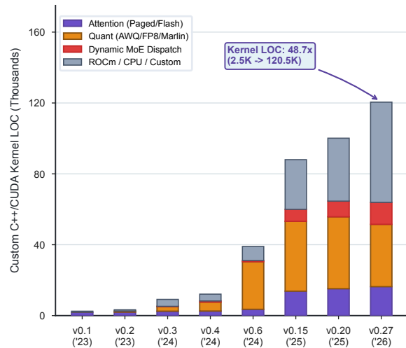
C. Inference Engine (vLLM) Application Kernel Fragmentation
