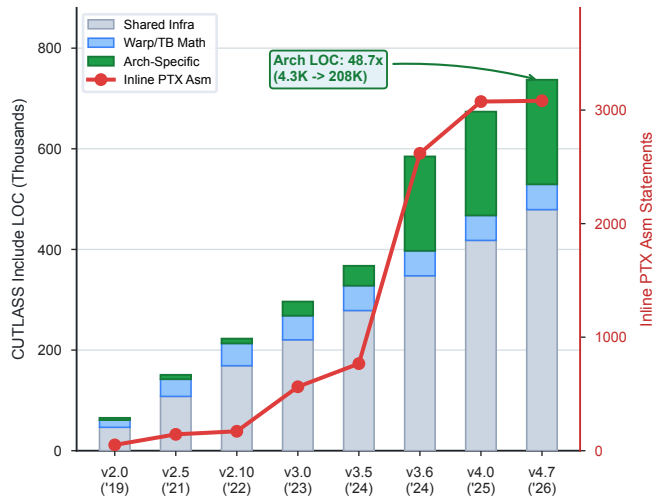
A. Hardware Primitives (CUTLASS) Explosive Low-Level Specialization
