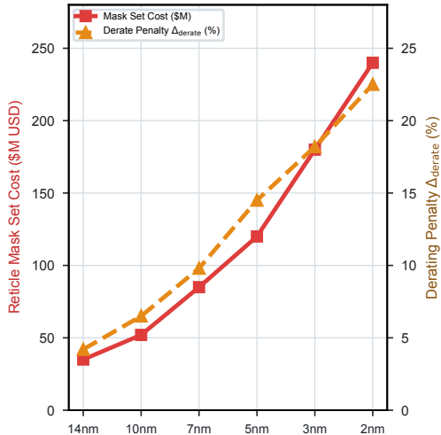
Panel C: Mask Cost vs Derating
