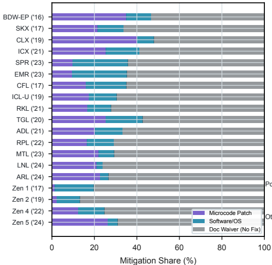
Panel A: Mitigation Pathways (19 CPUs)
