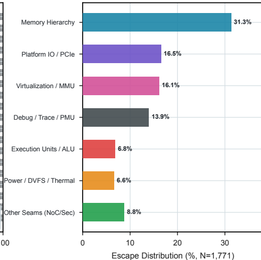
Panel B: Defect Concentration
