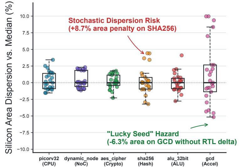
A: Area QoR Dispersion Across Logic Synthesis Pass Schedules B: Total Resource Footprint & Execution Jitter (150 Runs)
