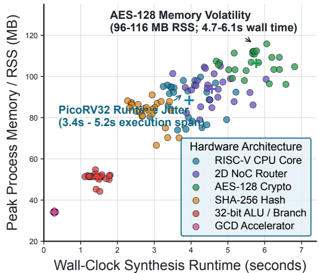
A: Area QoR Dispersion Across Logic Synthesis Pass Schedules B: Total Resource Footprint & Execution Jitter (150 Runs)
