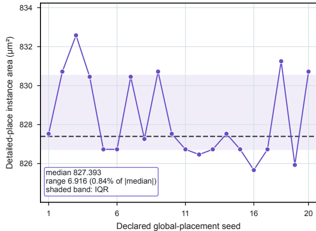
(a) Placement-Optimized Cell Area
