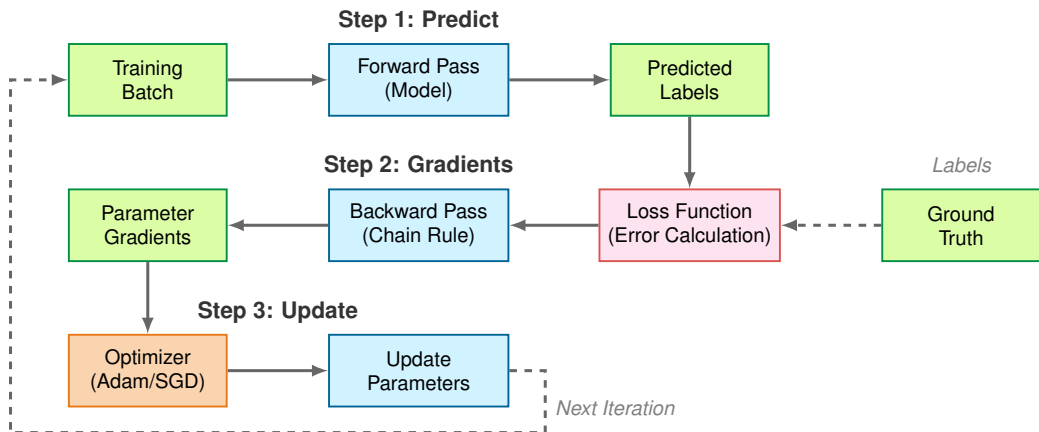
Figure 8.4: Training Loop: A single iteration flows through three steps—(1) forward pass from batch to predictions, (2) loss and gradients via backpropagation, and (3) optimizer update—with the dashed arrow returning to the next iteration.
