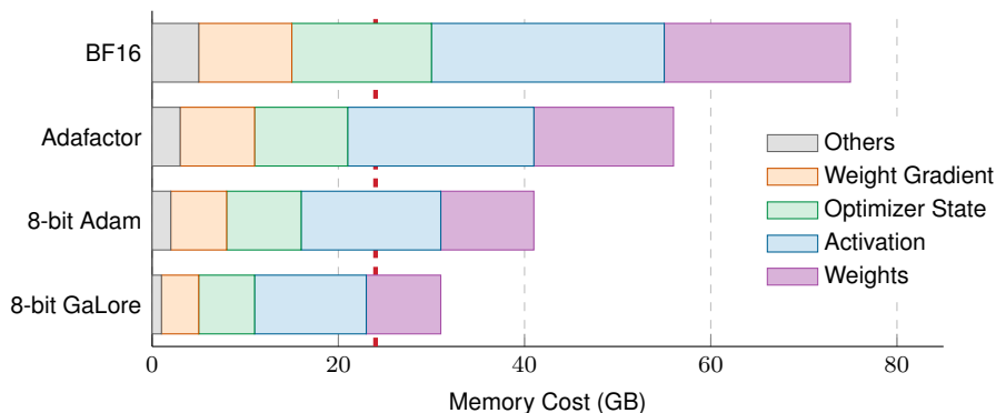
Figure 8.6: Memory Footprint Breakdown: Memory usage of a 7-billion-parameter LLaMA model across four memory-efficient optimizer configurations (BF16 Adam, Adafactor, 8-bit Adam, and 8-bit GaLoRE), decomposed into weights, activations, optimizer state, weight gradients, and other components. The dashed red line marks the RTX 4090 24 GB memory limit. Standard FP32 Adam (omitted from the bars; it requires well above 70 GB for this model) does not fit on a single 24 GB GPU; the bars compare the techniques that bring training back within budget, with 8-bit GaLoRE shrinking optimizer state most aggressively.
