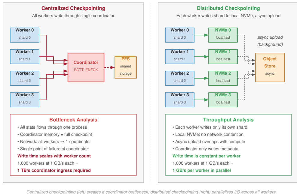
Centralized checkpointing (left) creates a coordinator bottleneck; distributed checkpointing (right) parallelizes I/O across all workers
