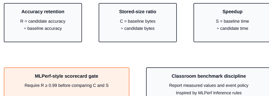
Figure 23.1: The MLPerf Optimization Olympics scorecard: one model, three axes, and a floor on accuracy that a submission must clear before its memory and latency numbers count.
