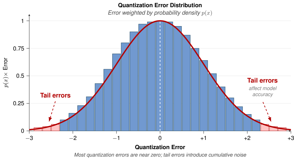
Figure 10.16: Quantization Error Distribution: Histogram of quantization error weighted by probability density p(x) , showing a bell-shaped curve centered near zero with tails that introduce quantization noise affecting model accuracy.
