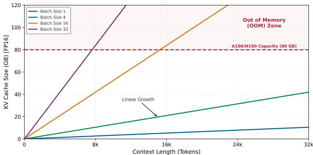
Figure 13.7: The KV-Cache Explosion: Memory usage vs. Context Length for a 70-billion-parameter-class model. Assumes 80 layers, d_{\text{model}} = 8192 , FP16 KV cache, GQA ( 8\times ). The linear growth of the Key-Value cache (storing attention history) quickly consumes available GPU memory (red dashed line). For batch size 32 (purple), the system hits the ‘OOM Zone’ at just 8k context length, forcing a trade-off between batch size (throughput) and context window (capability).
