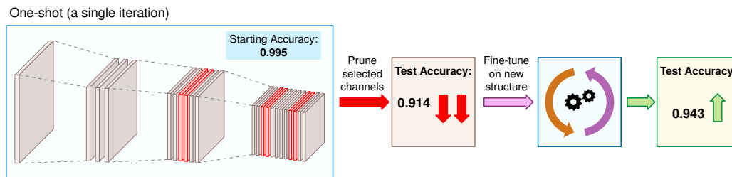
Figure 10.6: One-Shot Pruning Impact: All six channels (27 percent) are removed simultaneously, causing accuracy to drop from 0.995 to 0.914. Fine-tuning recovers only to 0.943, a 5 percent degradation compared to the 0.4 percent loss from iterative pruning, illustrating why gradual removal preserves accuracy more effectively.
