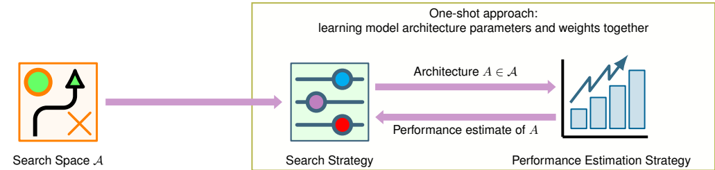
Figure 10.12: Neural Architecture Search Flow: Three components form a feedback loop: a Search Space defines candidate operations, a Search Strategy selects architectures, and a Performance Estimation Strategy evaluates each candidate. The strategy iterates by feeding performance estimates back into the search until convergence.
