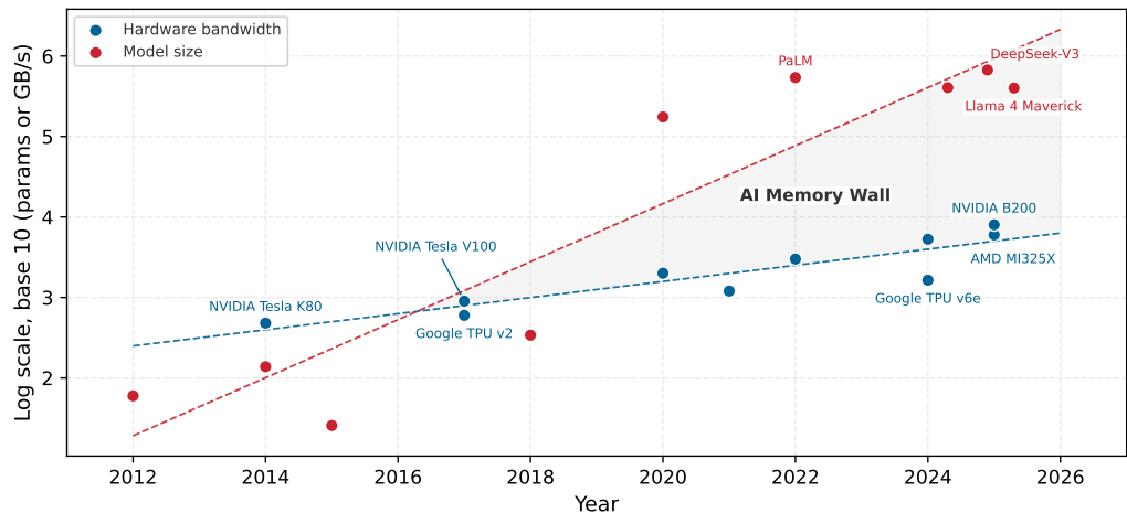
Figure 11.12: Model Size vs. Hardware Bandwidth: Publicly disclosed model parameter counts and hardware memory bandwidth plotted from 2012 to 2025, showing how model growth from AlexNet to hundred-billion-parameter models has far outpaced bandwidth improvements across GPU and TPU generations.
