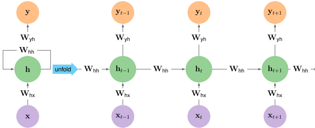
Figure 6.5: Recurrent Neural Network Unfolding: Left panel shows the compact recurrent loop; right panel unfolds this across time steps. Three weight matrices are shared across all steps: W_{hx} (input-to-hidden), W_{hh} (hidden-to-hidden), and W_{yh} (hidden-to-output). This weight sharing keeps parameter count constant at \mathcal{O}(d_{\text{hidden}}^2) regardless of sequence length. For a 128-dimensional hidden state, each time step requires 16,384 MACs for recurrent connections plus 12,800 for input projection.
