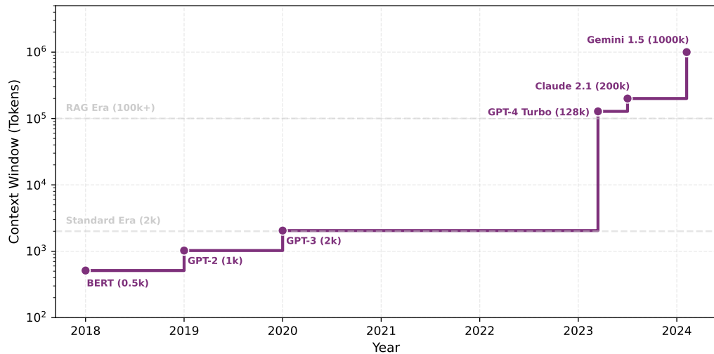
Figure 6.10: The Context Explosion: Maximum supported context window (tokens) over time (log scale). Values are representative public specifications at the time of announcement, not stable product guarantees. The transition from the standard era (2k) to the long-context era (100k) and beyond (1000k) represents a fundamental shift in how ML systems handle long-range dependencies: more of the relevant context can remain inside the model’s attention window, but the attention and KV-cache budgets grow with sequence length.
