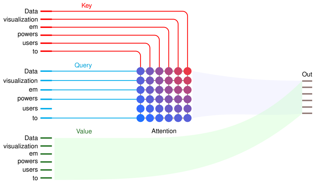
Figure 6.7: Query-Key-Value Attention Mechanism: For a 6-token sequence, queries (cyan) match against keys (red) to produce a 6 \times 6 attention matrix with \mathcal{O}(S^2) entries. Color intensity indicates attention weight: darker cells show stronger relationships. Each output position aggregates information from all values (green) weighted by its attention row. The matrix structure reveals both the computational pattern (thirty-six similarity computations) and the memory bottleneck (storing S^2 attention weights). Source: Transformer Explainer (Cho et al. 2025).
