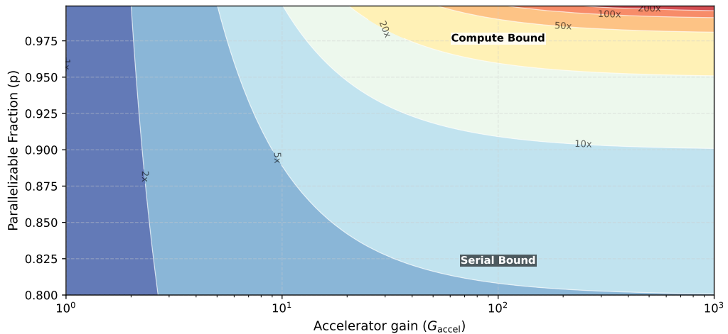
Figure 11.1: The Iron Law Heatmap: Total system speedup as a function of accelerator gain ( G_{\text{accel}} ) and parallel fraction ( p ). High speedup appears only near the top-right corner, where both accelerator gain and parallel fraction are high. The acceleration wall is the low- p region: if a workload is even slightly serial ( p < 0.9 ), increasing hardware speed yields little benefit. Contours span roughly 1\times – 500\times speedup.
