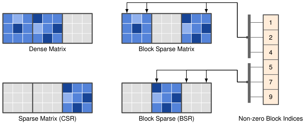
Figure 11.7: Sparse Storage Formats: Hardware efficiency depends on how sparse matrices are stored. The four panels show dense storage (simple but wasteful for zeros), CSR, block sparse, and the block-sparse BSR layout, which compress the matrix by storing only nonzero values plus the index of each stored block. The separate Non-zero Block Indices column is that index overhead: it is the price paid for skipping zeros, and structured sparsity (like N:M or blocks) keeps it predictable and compact so hardware can fetch data efficiently.
