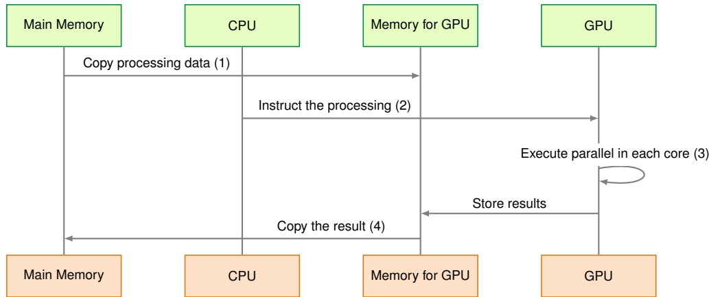
Figure 11.13: Host-Accelerator Data Transfer: AI workloads require frequent data movement between CPU memory and accelerators. The four sequential steps of copying input data, issuing execution instructions, parallel computation, and transferring results each introduce potential performance bottlenecks.
