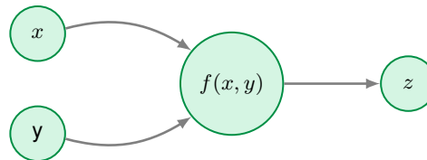
Figure 7.2: Simple Computational Graph: The computation z = f(x, y) represented as a graph, where nodes define operations and edges specify data flow.
