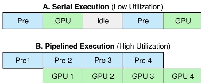
Figure 13.5: Request Pipelining: Pipelining hides latency by overlapping independent operations across different hardware resources. In pipelined execution (B), the CPU processes the next request’s data while the GPU executes the current request’s inference. This increases the GPU duty cycle toward 100 percent, effectively doubling or tripling throughput on the same hardware without changing the model.
