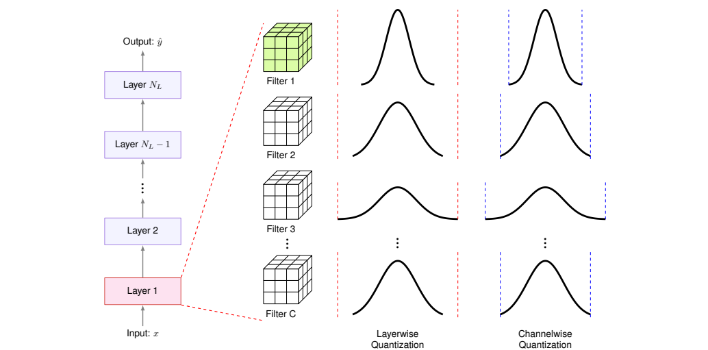
Figure 10.22: Quantization Range Variation: Different convolutional filters exhibit unique activation ranges, necessitating per-filter quantization to minimize accuracy loss during quantization. Adjusting the granularity of clipping ranges, as shown by the differing scales for each filter, optimizes the trade-off between model size and performance. Source: (Gholami et al. 2021a).
