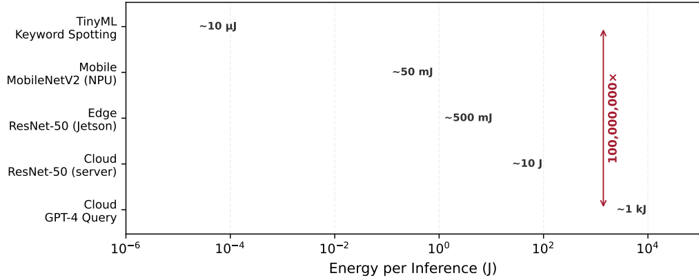
Figure 2.6: Energy Per Inference Across Deployment Paradigms: Full-system energy consumption per inference spans eight orders of magnitude, from ~10 μJ for TinyML keyword spotting to ~1 kJ for a cloud LLM query. This gap is not an engineering shortcoming—it reflects the physics of data movement, cooling, and network overhead that separates deployment tiers. The 100,000,000× difference explains why always-on sensing is only feasible at the TinyML tier.
