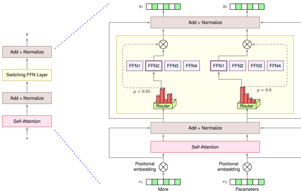
Figure 10.27: Conditional Computation: Switch transformers enhance efficiency by dynamically routing tokens to specialized expert subnetworks, enabling parallel processing and reducing the computational load per input. This architecture implements a form of mixture of experts where a gating network selects which experts process each token, allowing for increased model capacity without a proportional increase in computation. Source: (Fedus et al. 2022).
