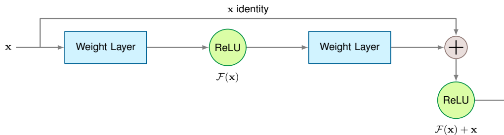
Figure 6.11: Residual Connection Block: The skip connection implements y = \text{ReLU}(\mathcal{F}(x) + x) , creating an identity shortcut that bypasses the weight layers before the final nonlinearity. During backpropagation, gradients flow through both the residual path (via \mathcal{F}'(x) ) and the identity path (via I before the final nonlinearity), helping gradients reach early layers even in 100+ layer networks. This architectural pattern enabled very deep residual CNNs and became central in transformer blocks and many other modern architectures.
