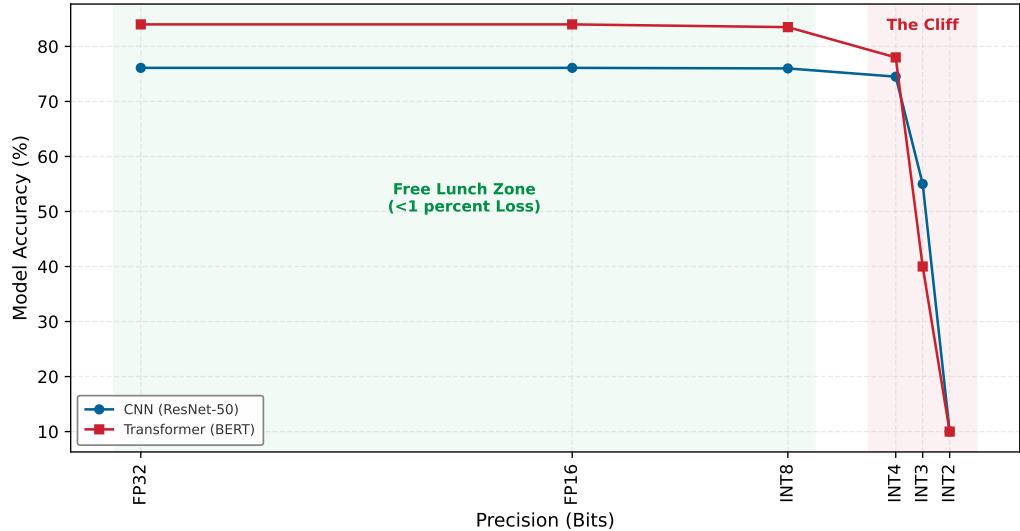
Figure 10.13: The Quantization Free Lunch: Model accuracy vs. Bit-width. Most models exhibit a ‘Free Lunch’ plateau where reducing precision from FP32 to INT8 yields <1 percent accuracy loss. This robustness collapses at the ‘Quantization Cliff’ (typically 3–4 bits). Curves are illustrative and meant to show qualitative behavior.
