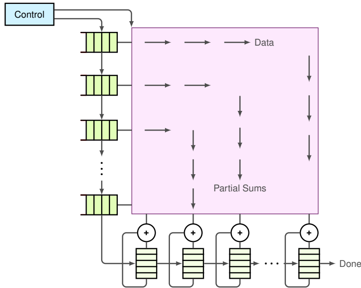
Figure 11.8: Systolic Array Dataflow: A control unit feeds input data streams into a grid of processing elements, each performing multiply-accumulate operations. Data flows horizontally and vertically through the array in a pipelined manner, maximizing operand reuse and minimizing memory access, as exemplified by Google’s TPUv4.
