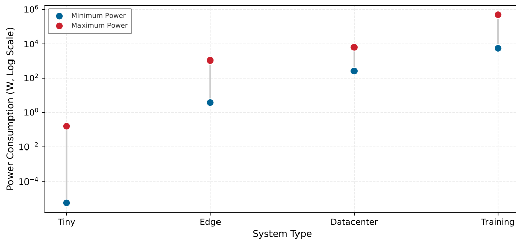
Figure 12.6: Power Consumption Differentials: Power usage spans over ten orders of magnitude across ML system types, from microwatts in tinyML devices through watts at the edge to kilowatts in data center inference and hundreds of kilowatts for training clusters. Ranges are representative and vary by hardware and workload.
