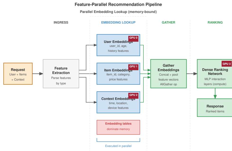
Figure 10.6: Feature-Parallel Batching Pipeline: Requests are batched by feature type (Users, Items, Context) and dispatched to specialized embedding servers in parallel. The retrieved embeddings are then concatenated and processed by the dense ranking head. This architecture enables scaling to trillions of parameters by decoupling embedding storage from dense compute.
