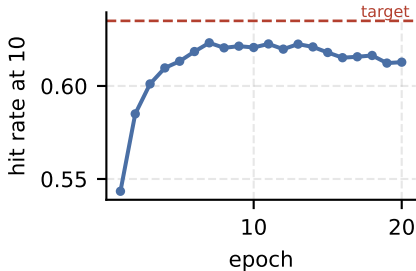
recommendation
