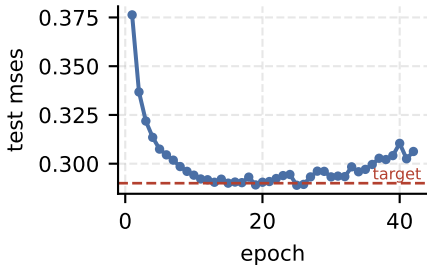
time-series-forecasting
