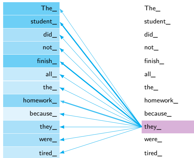
Figure 6.6: Illustrative Attention Pattern: A schematic attention pattern for the pronoun “they.” Line thickness represents hypothetical attention-weight magnitude, with stronger links to “student,” “finish,” and “homework.” One attention layer connects all positions directly and can compute their dense interactions in parallel.
