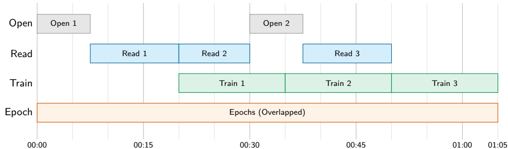
Figure 8.11: Illustrative Overlapped Data Prefetching: File-open and read work overlaps accelerator training while preserving the same individual stage durations as the serial schedule. The schematic schedule spans approximately 65 min, compared with 95 min for the serial schedule.
