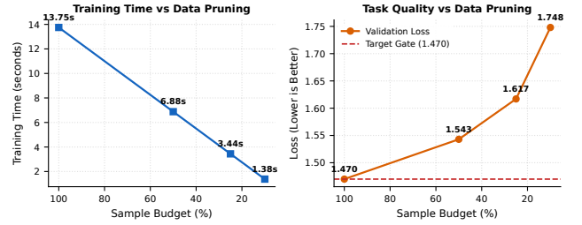
Figure 5. Data Lens quality-efficiency trade-off. Pruning sample budgets (100% \rightarrow 10%) achieves linear wall-clock speedup (13.75s \rightarrow 1.38s) alongside quality degradation under inherited target criteria.
