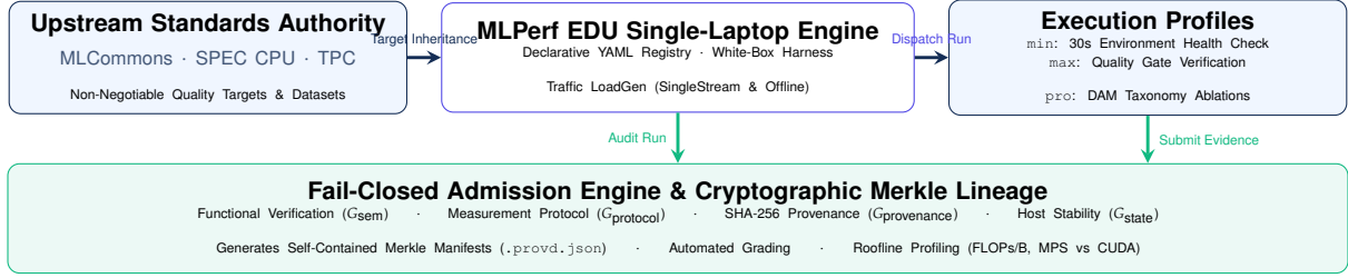
Figure 1. MLPerf EDU system architecture. Industrial MLCommons quality targets and evaluation protocols are inherited without local discretion, executed across three profiles (min, max, pro), and audited by a fail-closed admission engine to generate self-contained Merkle provenance digests.
