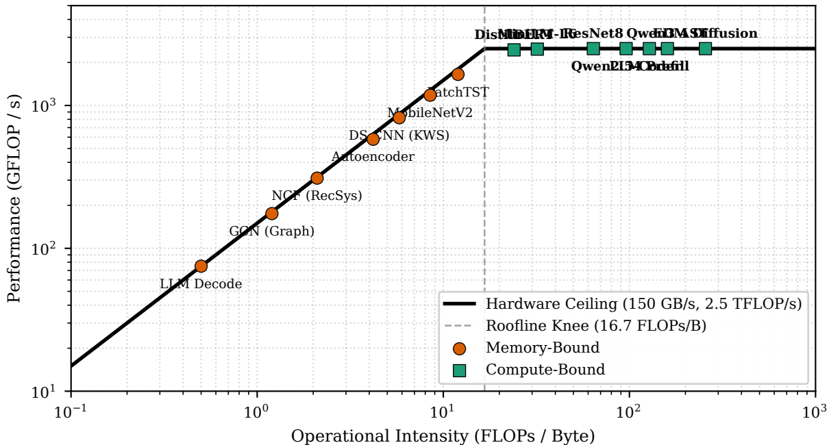
Roofline Model: Operational Intensity & Hardware Ceilings across 14 Workload
