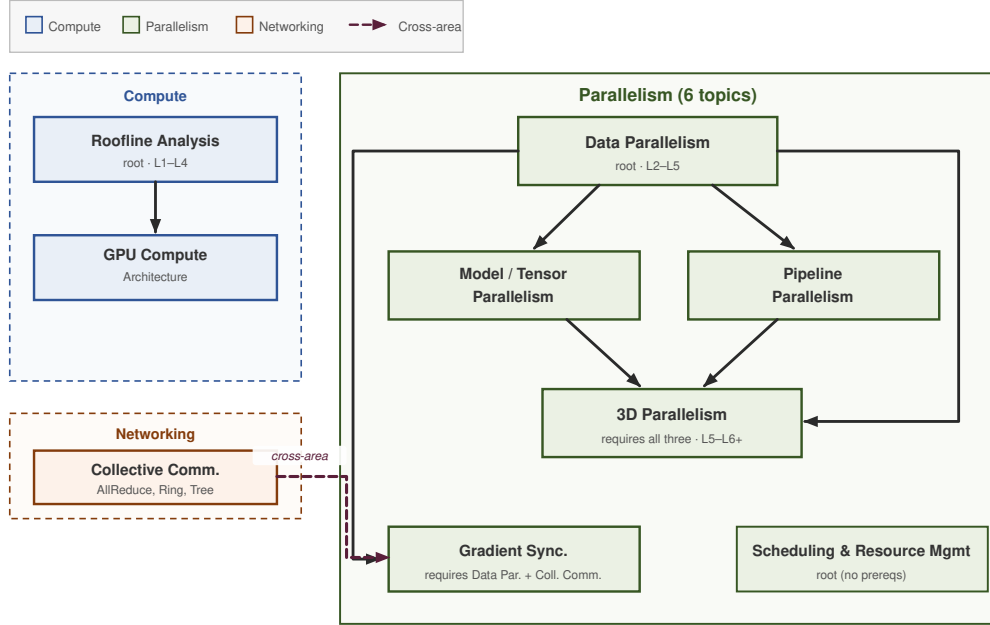
Figure 5. Prerequisite subgraph: parallelism area. Six of 88 topics showing the dependency diamond: Data Parallelism fans out to Model/Tensor Parallelism and Pipeline Parallelism, which converge on 3D Parallelism. The dashed cross-area edge from Collective Communication (networking) to Gradient Synchronization illustrates how the prerequisite graph connects competency areas. The full graph has 57 edges, maximum depth 4, and is verified acyclic.
