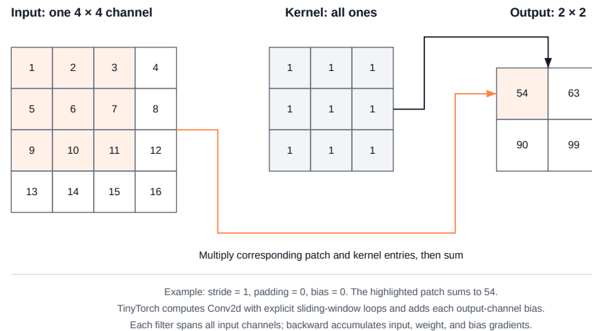
Figure 9.1: One filter, four windows: The highlighted input patch supplies the first output. Moving the same kernel across the remaining positions produces the other three values.
