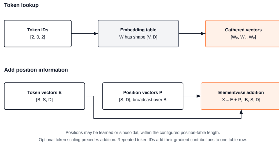
Figure 11.1: The embedding pipeline. A token ID selects one row of the embedding table; the row for that token’s position is added; the sum is the vector the rest of the network sees.
