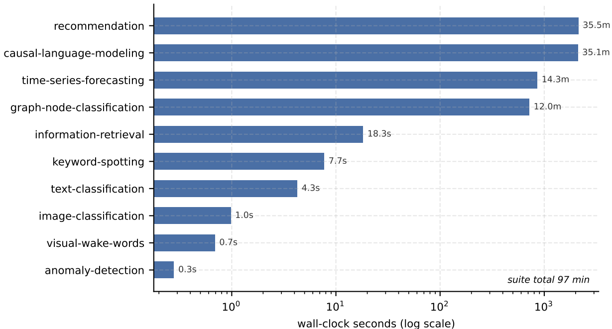
Measured runtime of the canonical max path
