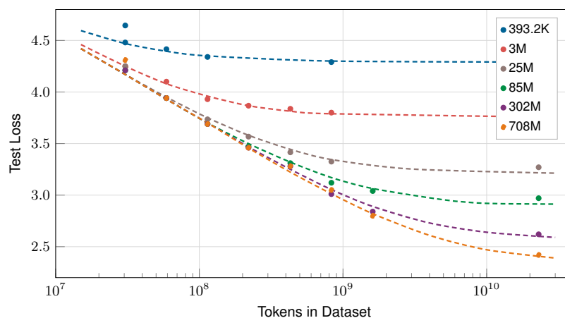
Figure 1.8: Loss vs. Dataset Size Across Model Scales: Test loss curves showing how models of different sizes (393K to 708M parameters) benefit from increased training data. Larger models achieve lower loss but all curves exhibit diminishing returns at high token counts.
