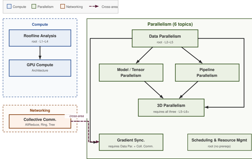
Figure 5. Prerequisite subgraph: parallelism area. Six of 89 topics showing the dependency diamond: Data Parallelism fans out to Model/Tensor Parallelism and Pipeline Parallelism, which converge on 3D Parallelism. The dashed cross-area edge from Collective Communication (networking) to Gradient Synchronization illustrates how the prerequisite graph connects competency areas. The full graph has 57 edges, maximum depth 4, and is verified acyclic.
