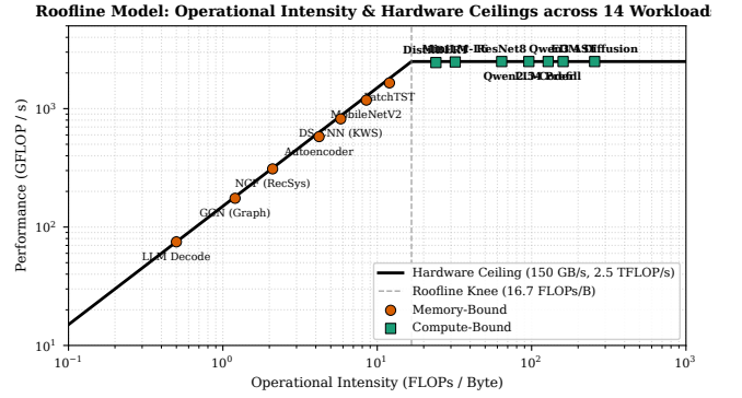
Figure 5. Roofline visual performance model across all 14 workload. Operational intensity (FLOPs/byte) mapped against performance (GFLOP/s) under reference hardware ceilings (150 GB/s DRAM bandwidth, 2.5 TFLOP/s compute peak). The knee point at 16.7 FLOPs/byte separates memory-bandwidth bound workloads (e.g., LLM Decode, GCN ogbn-arxiv, NCF recommendation) from compute-bound GEMM workloads (e.g., LLM Prefill, ResNet8, EDM diffusion).
