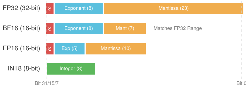
Figure D.3: Numerical Format Bit Layouts: A visual comparison of bit allocations. Note how BF16 (Brain Float 16) preserves the 8-bit exponent of FP32, ensuring the same dynamic range for training stability. FP16 trades range for precision, often requiring loss scaling to prevent underflow.
