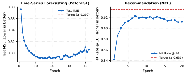
Figure 2. Convergence behavior of training workloads. Per-epoch quality metrics against inherited target gates showing seed sensitivity and convergence limits.
