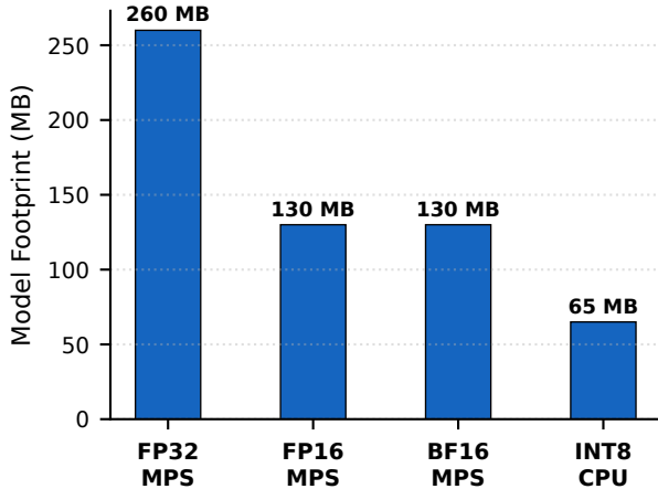
DistilBERT Weight Footprint
