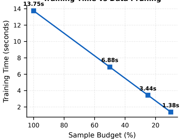
Training Time vs Data Pruning
