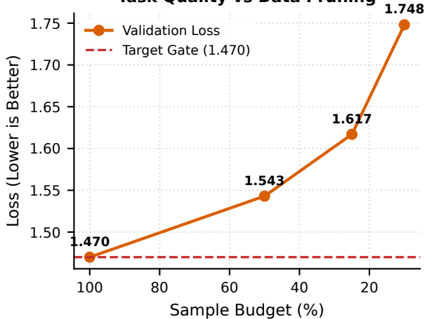
Task Quality vs Data Pruning
