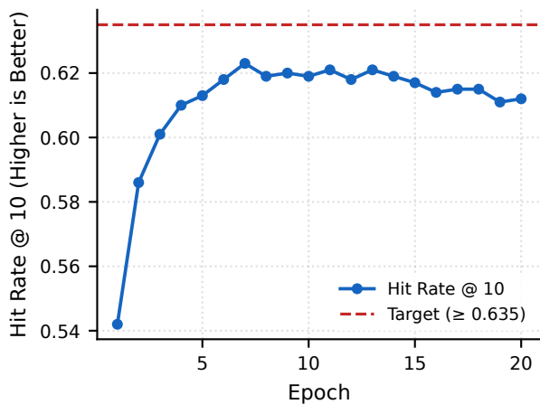
Recommendation (NCF)
