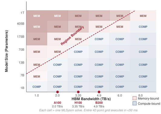
Figure 5: Design-Space Exploration: Bottleneck Regime Map. Each cell shows the binding constraint (memory or compute) for a given model size and HBM bandwidth combination under FP16 training at batch size 256. Larger models with lower bandwidth are memory-bound; smaller models with higher bandwidth are compute-bound. The diagonal regime boundary shifts as hardware generations increase bandwidth (A100 → H100 → B200). The entire 42-point grid executes in <50 ms.
