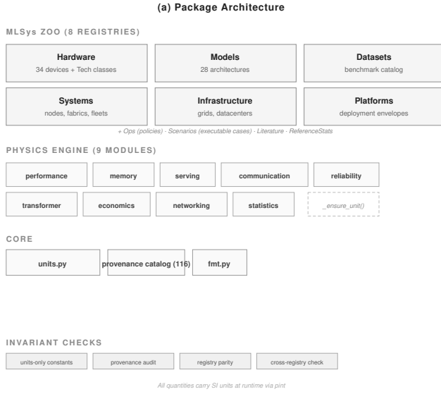
Figure 3: System Anatomy. (a) Package architecture: eight registries (six shown) provide typed, provenance-tracked specifications, nine physics modules supply domain-aligned formulas, and four invariant checks enforce design decisions as the codebase evolves. (b) Analysis pipeline: a workload lowers to a hardware-agnostic intermediate representation; four input layers feed 28 stateless resolvers organized in three tiers; the output is a three-level SystemEvaluation scorecard (Feasibility, Performance, Macro).
