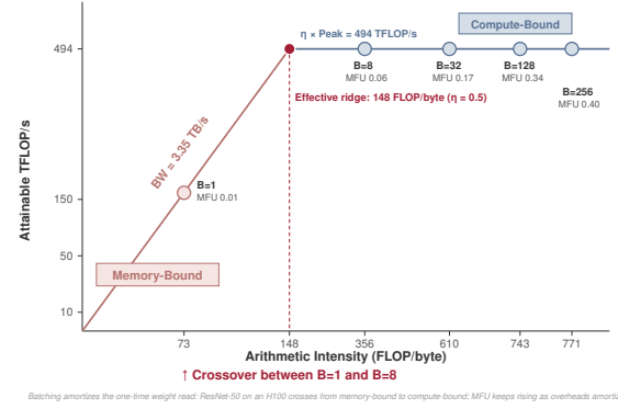
Figure 6: Roofline Crossover: ResNet-50 Batch Size Sweep on H100. Increasing batch size moves the operating point rightward along the Roofline, transitioning from memory-bound (red) to compute-bound (blue) between batch 1 and batch 8. The peak ridge point is 989/3.35 \approx 295 FLOP/byte; at \eta = 0.5 the effective ridge sits at \approx 148 FLOP/byte. MFU continues rising past the crossover as dispatch and framework overheads amortize.
