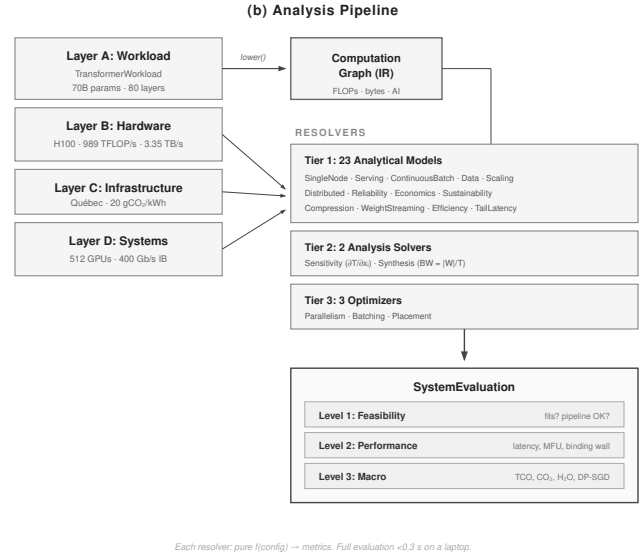
Figure 3: System Anatomy. (a) Package architecture: eight registries (six shown) provide typed, provenance-tracked specifications, nine physics modules supply domain-aligned formulas, and four invariant checks enforce design decisions as the codebase evolves. (b) Analysis pipeline: a workload lowers to a hardware-agnostic intermediate representation; four input layers feed 28 stateless resolvers organized in three tiers; the output is a three-level SystemEvaluation scorecard (Feasibility, Performance, Macro).
