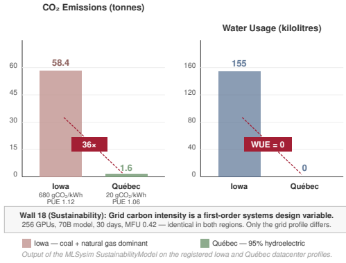
Figure 7: Geography as a Systems Variable: Iowa vs. Québec. An identical 256-GPU cluster training a 70B model for 30 days produces 36 \times more CO 2 in Iowa (coal/gas grid circa 2020, 680 gCO 2 /kWh, PUE 1.12) than in Québec (95% hydroelectric, 20 gCO 2 /kWh, PUE 1.06): 58.4 vs. 1.6 tonnes. Water usage diverges even more sharply because Québec’s registered WUE is zero. Hardware, model, parallelism strategy, and MFU are identical; only the regional grid profile differs between the two sites.
