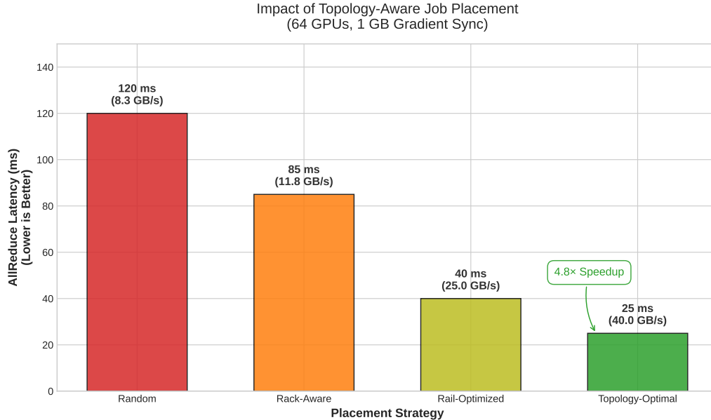
Figure 8.4: Topology Placement Impact: AllReduce latency across four placement strategies (Random, Rack-Aware, Rail-Optimized, and Topology-Optimal) for a 1 GB gradient sync on 64 GPUs. Topology-aware scheduling reduces sync latency from 120 ms to 25 ms, yielding a 4.8 \times speedup.
