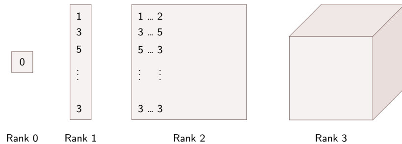
Figure 7.8: Tensor Rank Hierarchy: Ascending tensor ranks (0 to 3) generalize multi-dimensional indexing from scalars to volume tensors. Each additional rank adds an organizational axis that the framework must linearize into physical memory addresses via strides.
