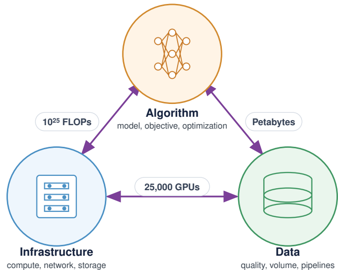
Figure 1.14: The AI Triad at Scale: The three interdependent components of every ML system. At production scale, each component’s requirements intensify: data pipelines must handle petabytes with consistent quality; algorithms can demand 10^{25} FLOPs for large-model training; and infrastructure must coordinate thousands of accelerators while maintaining fault tolerance. Changes to any vertex cascade through the others, creating the multi-dimensional optimization challenge that defines ML systems engineering.
