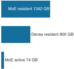
MoE keeps every expert resident but activates few per token.
