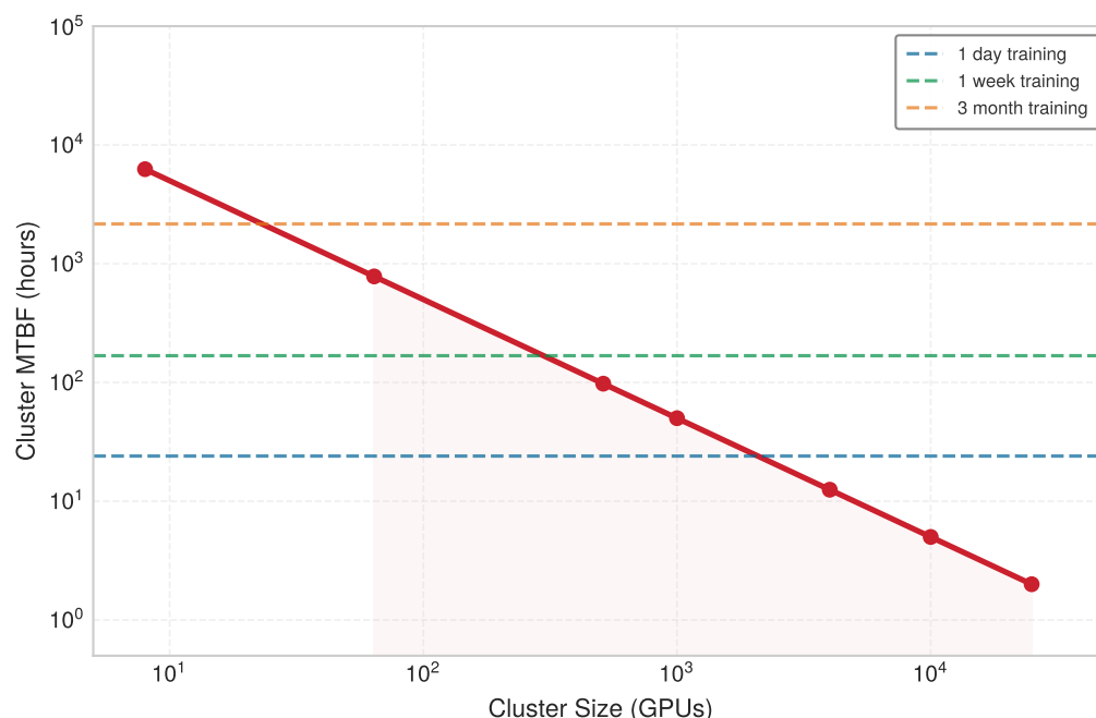
Figure 7.2: The Reliability Gap: As GPU count increases, cluster MTBF drops below common training durations. A 10,000-GPU cluster experiences a failure roughly every 5 hours, making a 3-month training run impossible without fault tolerance mechanisms.
